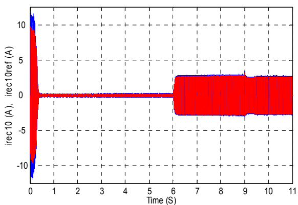
Fig. 8 The network current i_{rec10} and its reference
