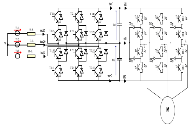
Fig. 1 Back-to-back three-level converters-Induction motor
