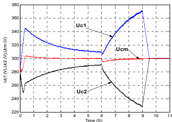
Fig. 7 DC bus capacitors voltages
