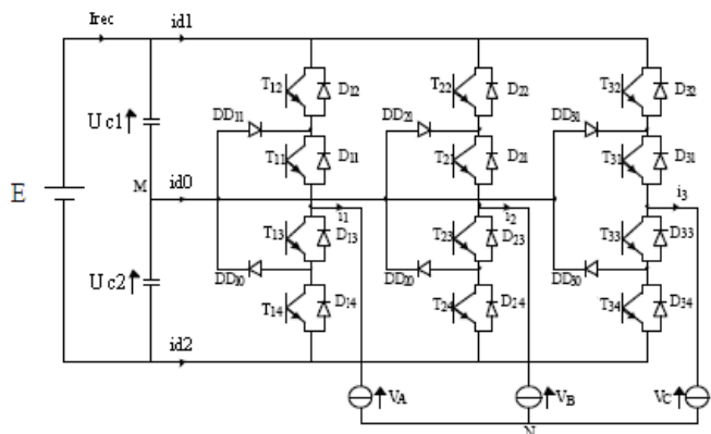
Fig. 5 Three-level NPC voltage source inverter
