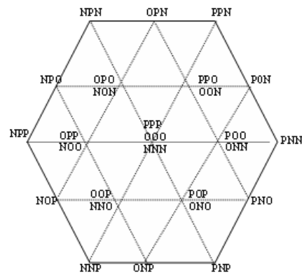
Fig. 3 Space vector diagram of a three-level inverter
