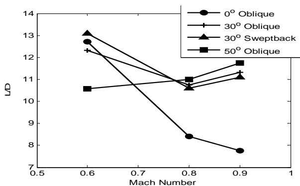
Fig. 3 Lift-to-Drag ratio curve against Mach number
