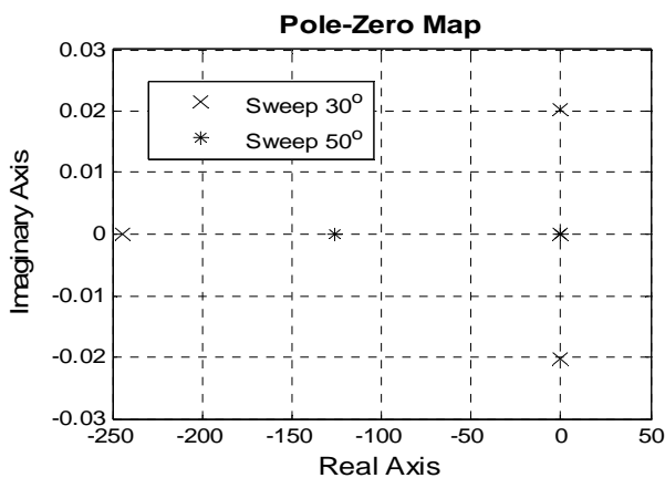
Fig. 5 Eigenvalues for 30° and 50° sweep at Mach 0.9
