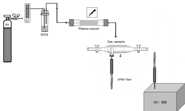
Fig. 2 Cold plasma system for BTEX removal
