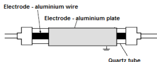
Fig. 1 Plasma reactor with annular cylindrical electrodes
