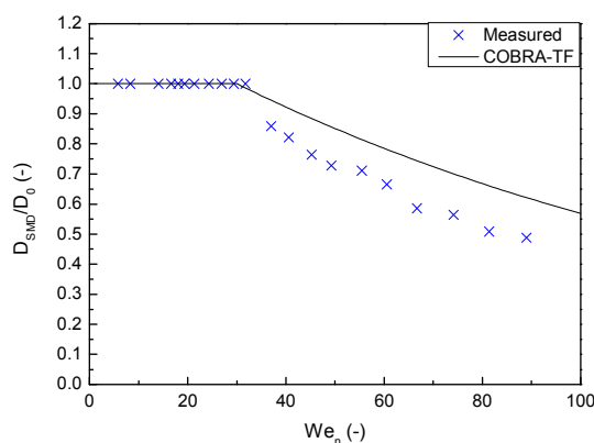
Fig. 4 Droplet Breakup
