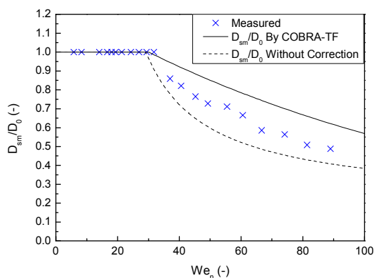
Fig. 8 Measured Data with New Model
