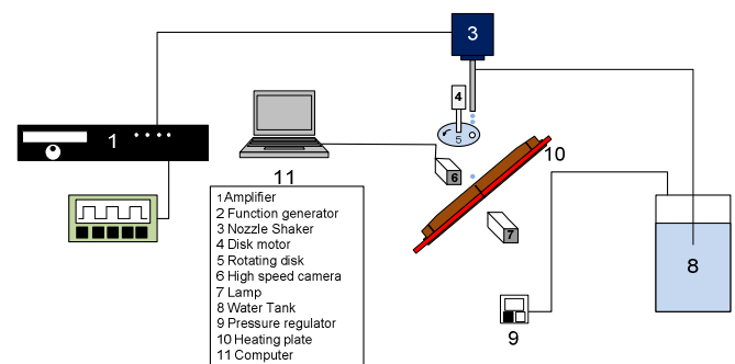
Fig. 2 Experimental Apparatus
