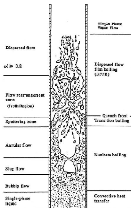
Fig. 1 Two Phase Flow Regime in flooding Scenario
