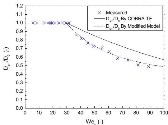
Fig. 10 Adjusted Correction Factor
