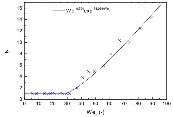
Fig. 6 Secondary Droplet Number
