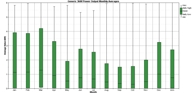
Fig. 7 Monthly output power of wind generator
