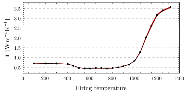
Fig. 6 Thermal conductivity of the fired samples
