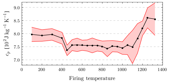
Fig. 10 Specific heat capacity of the fired samples
