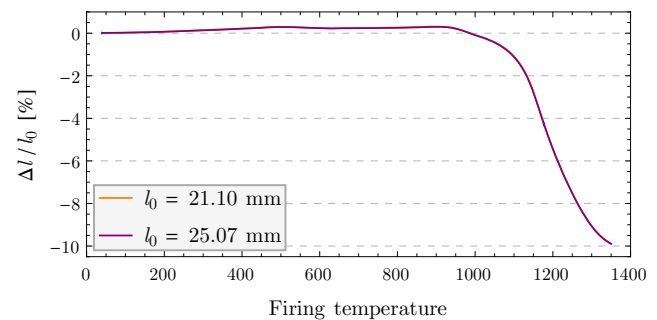
Fig. 8 Dilatometry performed on 2 samples
