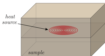
Fig. 1 Basic principle (model) of the TPS method
