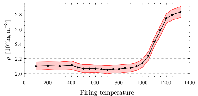
Fig. 7 Bulk density of the fired samples
