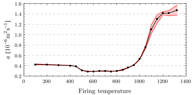
Fig. 5 Thermal diffusivity of the fired samples
