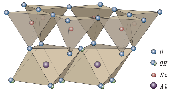
Fig. 4 Structure of the kaolinite
