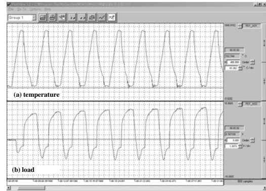
Fig. 3 An example of temperature control and load monitoring at the initial stage of thermal fatigue test conducted under 200-800°C temperature cycles
