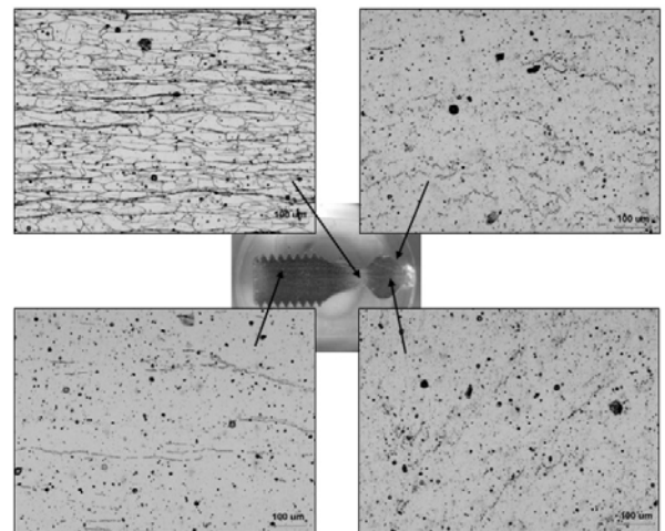
Fig. 8 Microstructure of STS 304 specimen tested under 200-900°C thermal cycles
