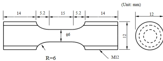
Fig. 3 Dimensions of specimen used in this study
