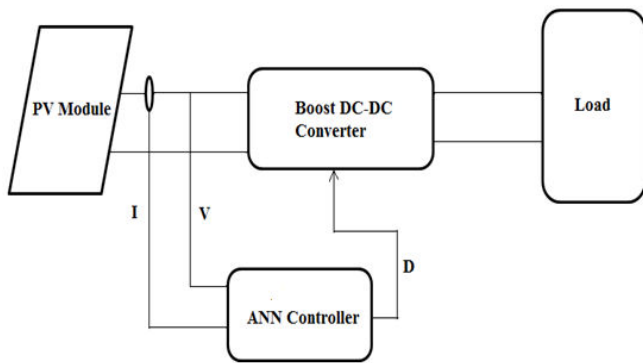
Fig. 4 Block diagram of the PV system with the proposed MPPT controller.
