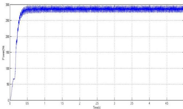
Fig. 10 Output Power Waveform of Hill-Climbing Algorithm
