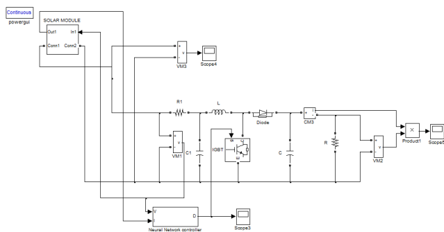
Fig. 6 Simulation Circuit of Proposed System
