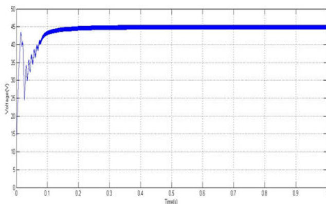
Fig. 7 Voltage from Solar Panel
