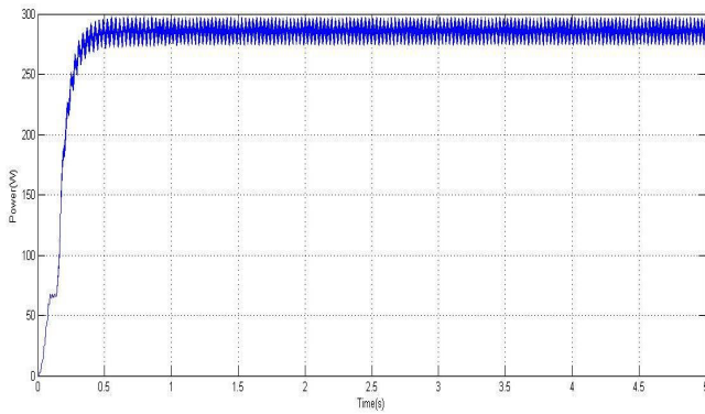
Fig. 3 PV output power of the hill-climbing method
