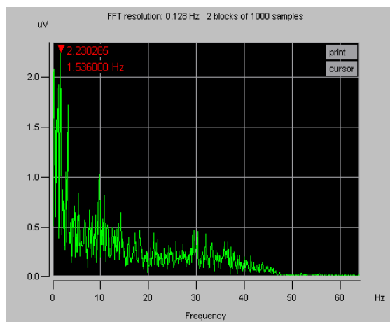
Fig. 4 Power spectrum during eye blink
