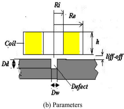
Fig. 1 Description of the configuration geometry (plate, probe, defect)
