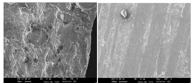
Fig. 4 SEM microstructure of drilled surface at a cutting speed 150.72m/min (a) 0.25mm/rev, (b) 0.05mm/rev
