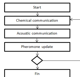
Fig. 1 Model of Ant Colony Optimization with Acoustic Communication
