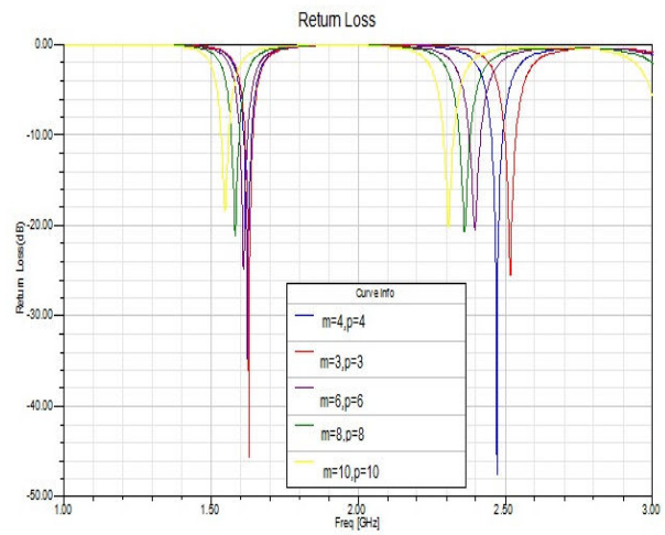
Fig. 6 Simulated return loss for different values of ' m ' & ' p '
