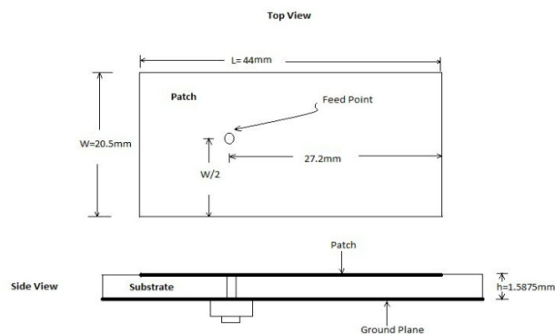
Fig. 2 Schematic diagram of antenna
