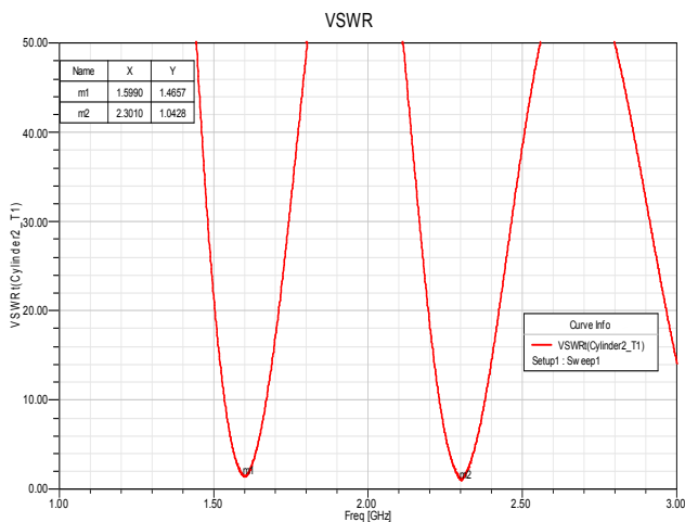
Fig. 4 (b) Simulated VSWR against freq. for antenna1
