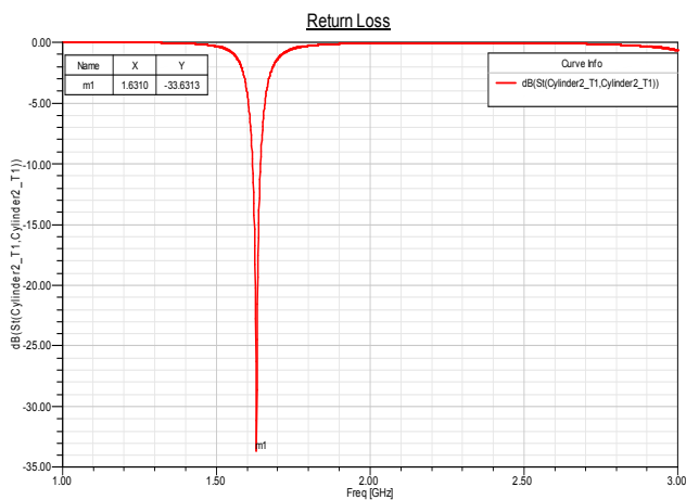
Fig. 4 (a) Simulated return loss for antenna 1
