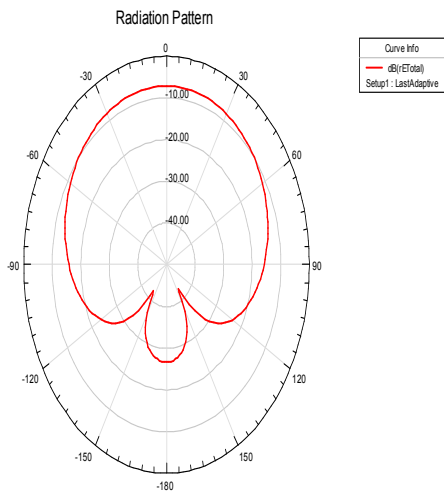
Fig. 5 (b) E-plane radiation pattern for proposed antenna
