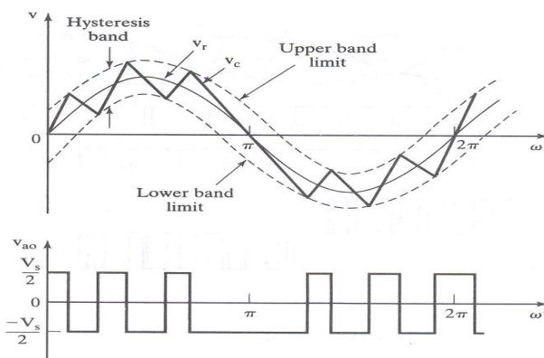
Fig. 8 Delta modulation
