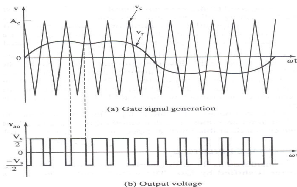
Fig. 7 Harmonic injected modulation
