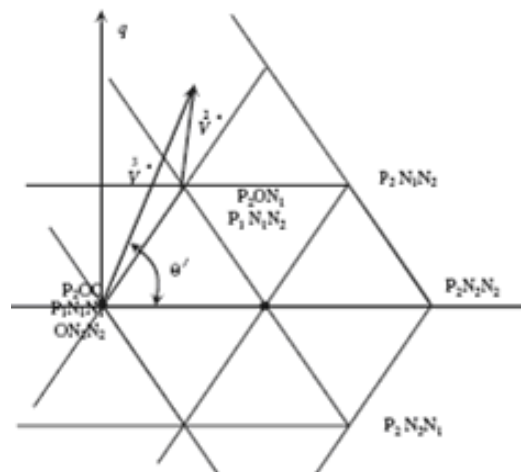
Fig. 15 Second Translation of Reference Voltage Vector
