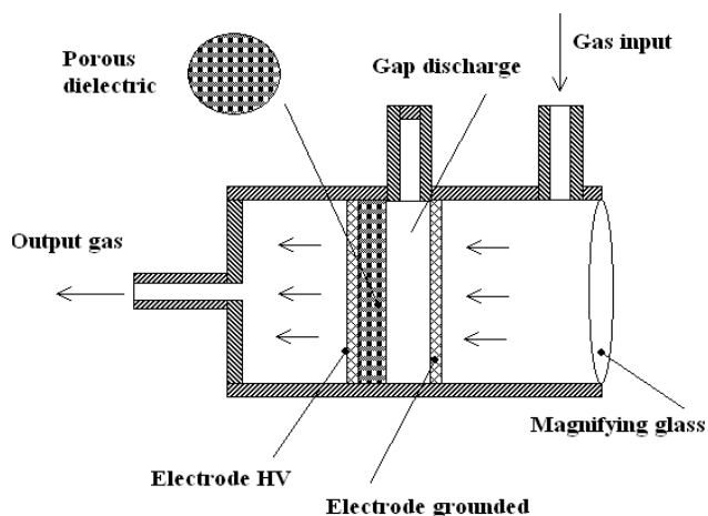
Fig. 3 Configuration of reactor with porous dielectric
