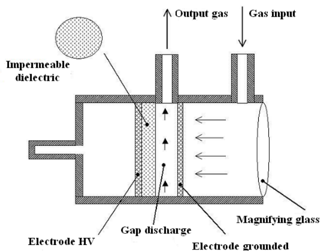
Fig. 4 Configuration of reactor with impermeable dielectric
