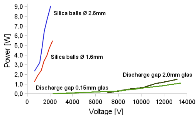
Fig. 9 Dependency of discharge power on input voltage
