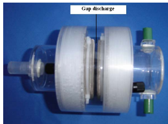
Fig. 1 Plasma reactor with mesh electrodes
