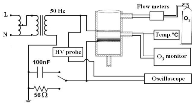
Fig. 2 Schematic measurement system
