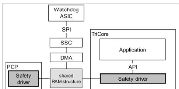
Fig. 2 The SafeTcore driver system structure
