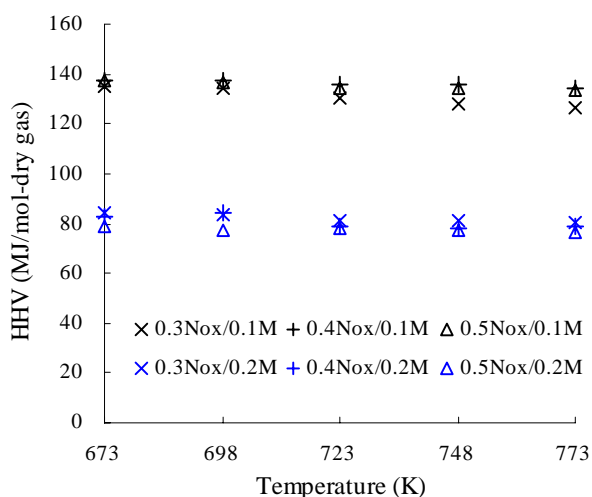
Fig. 6 HHV of dry product gas
