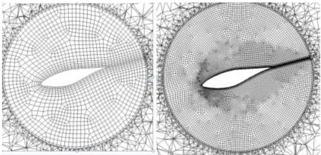
Fig. 4 Two kinds of Mesh distributions
