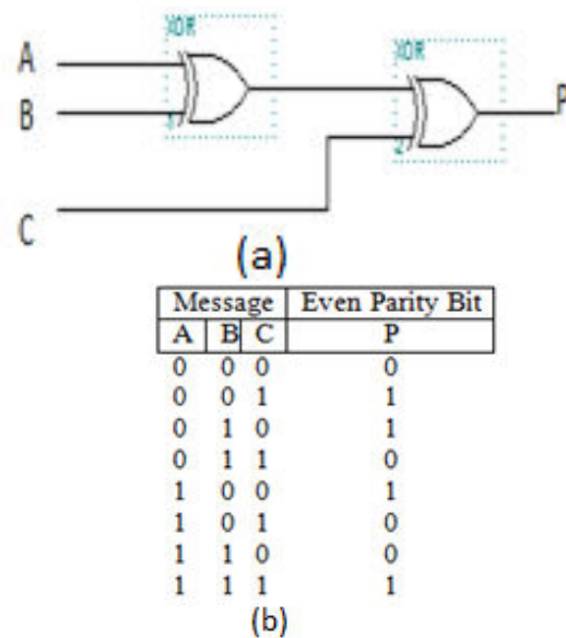
Fig. 11 Parity Generator (a) Parity generator using XOR gate (b) Input and output vector
