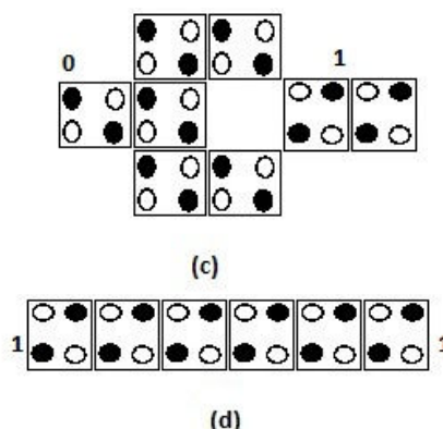
Fig. 3 (a) QCA AND gate, (b) QCA OR gate, (c) QCA inverter gate and (d) QCA bus
