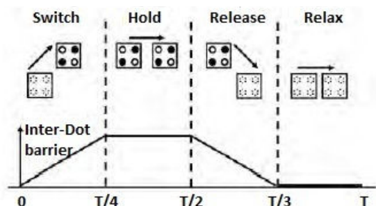
Fig. 4 Four phases QCA Clocking
