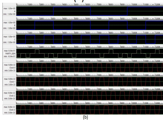
Fig. 12 Even Parity generator layout and Simulation results
