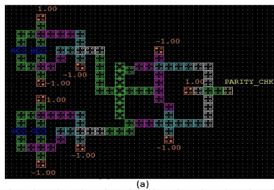
Fig. 13 Parity Checker (a) Parity Checker using XOR gate (b) Input and output vector
