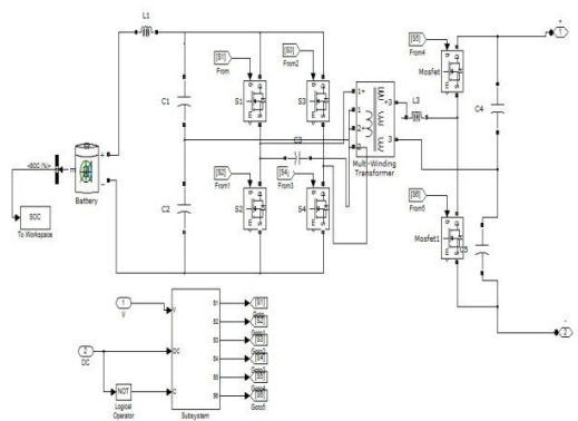
Fig. 6 Model of Bidirectional boost converter
