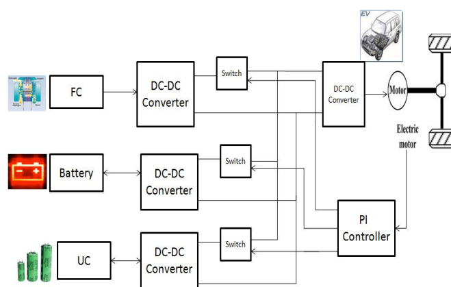
Fig. 1 Proposed System of a hybrid electric vehicle
