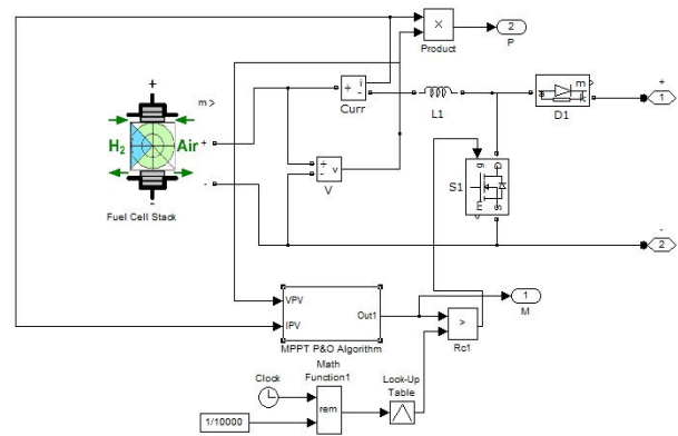
Fig. 5 PEMFC with boost converter
