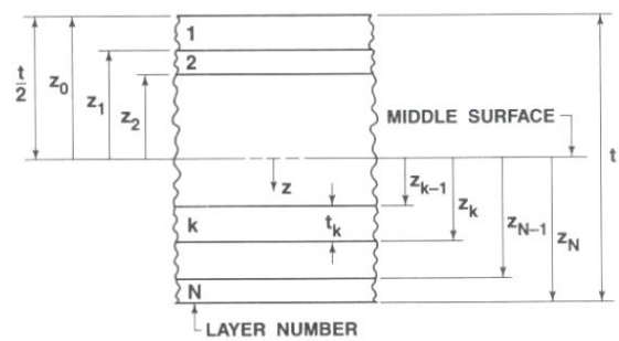
Fig. 3 Geometry of an N-layered laminate
