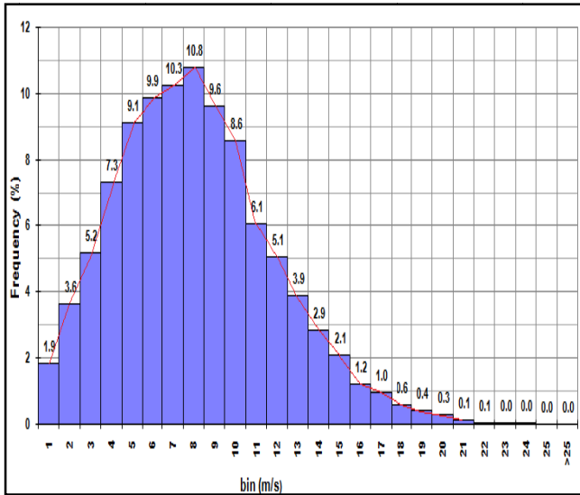
Fig. 4 Wind Speed Distribution 40m
