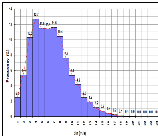
Fig. 2 Wind Speed Distribution
