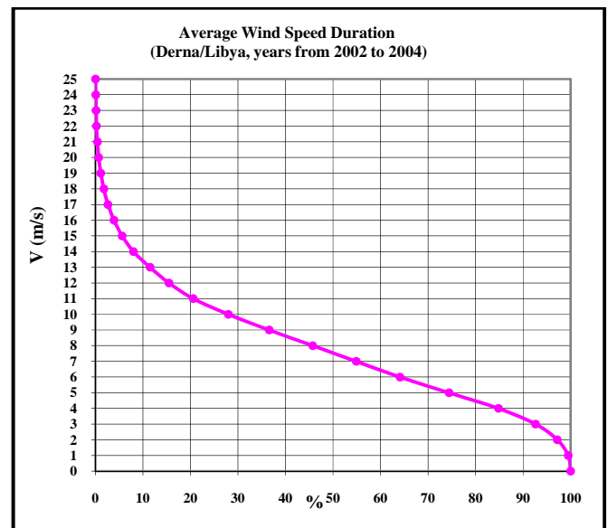
Fig. 10 Duration of Average Wind Speed
