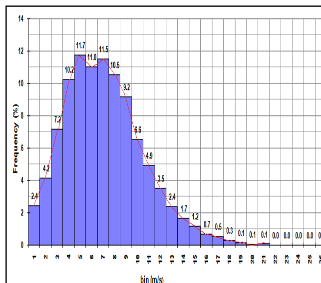
Fig. 3 Wind Speed Distribution 20m
