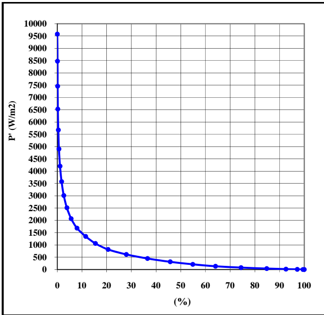
Fig. 11 Specific Power Durations Darnah- Libya
