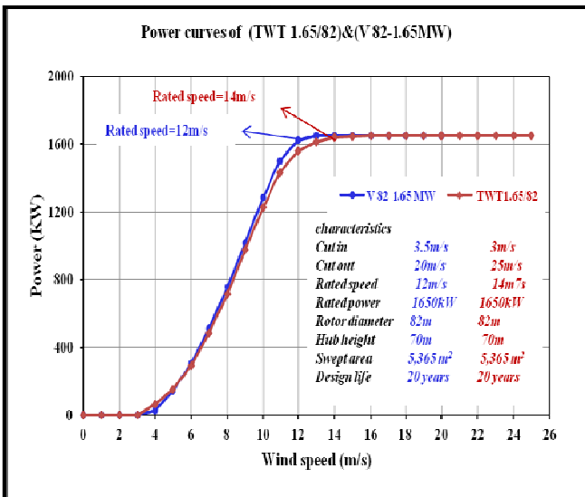
Fig. 12 Power Curves Of (TWT 1.65/82) & (V82-1.65MW)
