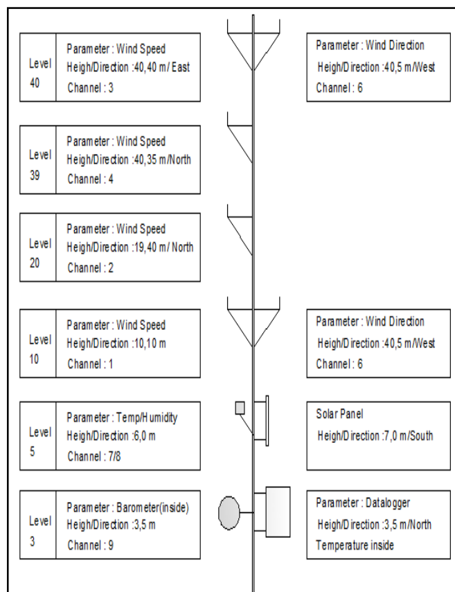
Fig. 1 Meteorological Mast in the El-Maqrn station
