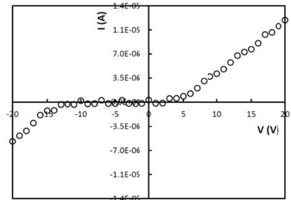
Fig. 6 Current-voltage characteristics of a Sn nanocluster device
