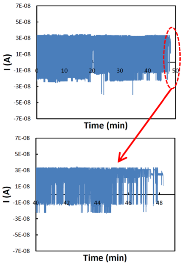
Fig. 5 The electric current through a Sn nanocluster device using V = 0.1 V
