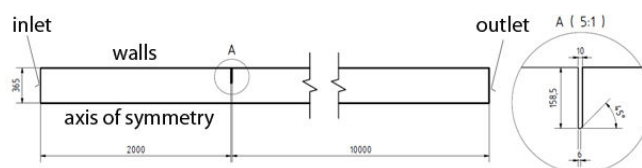
Fig. 2 Geometry of the model
