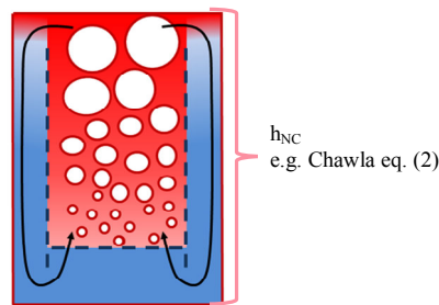
Fig. 2 Natural circulation flow in boiling pools
