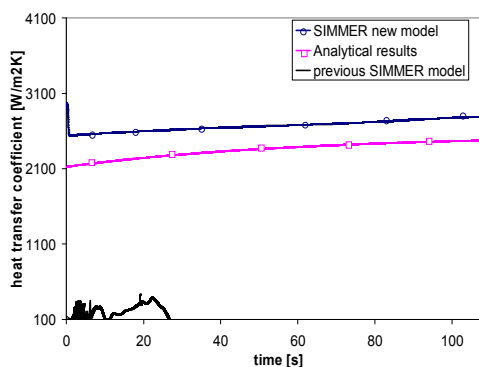
Fig. 4 Liquid-structure heat transfer coefficient for simple case test (one radial mesh nodalization)
