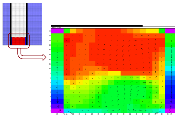
Fig. 6 Mesh scheme following the boundary layer thickness of the colder fluid returning in a heated pool
