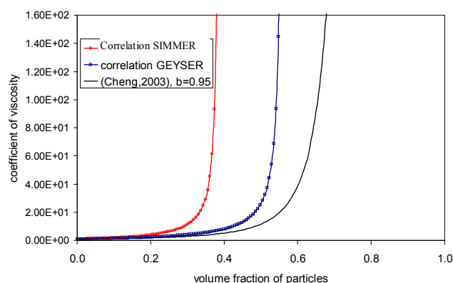
Fig. 10 Different particle-fluid effective viscosity multiplication coefficients
