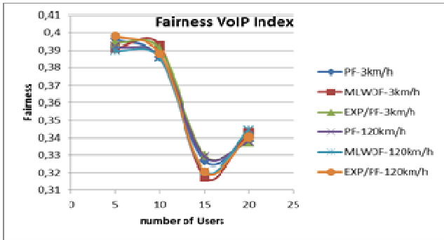
Fig. 16 Fairness for voip flows
