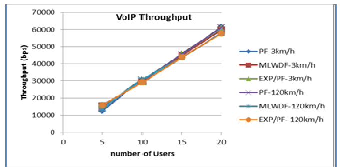
Fig. 14 Throughput for voip flows
