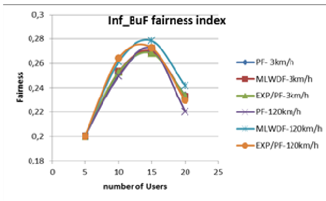
Fig. 8 Fairness for best effort flows
