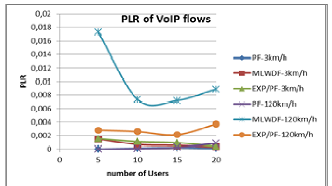
Fig.15 Packet Loss Ratio for voip flows
