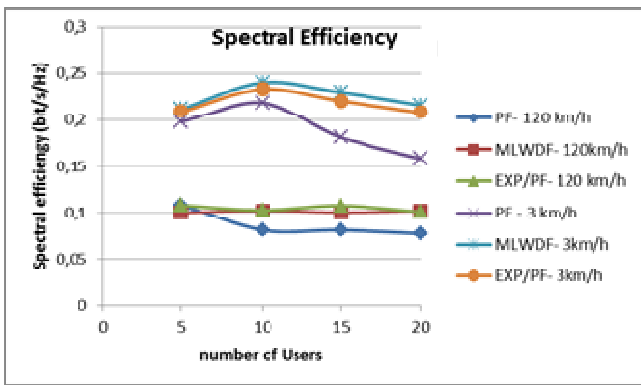
Fig. 17 Spectral efficiency
