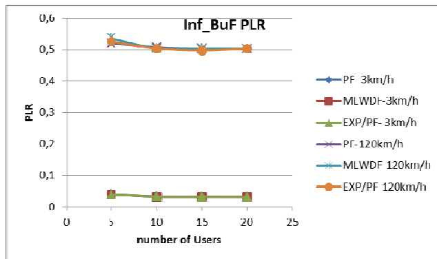
Fig. 7 Packet Loss Ratio for best effort flows
