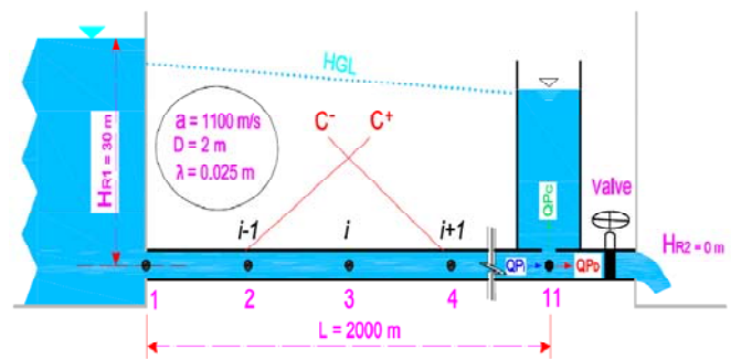
Fig. 11 Simple reservoir valve system
