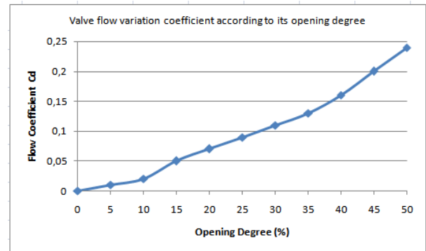
Fig. 10 Valve flow variation coefficient according to its opening degrees
