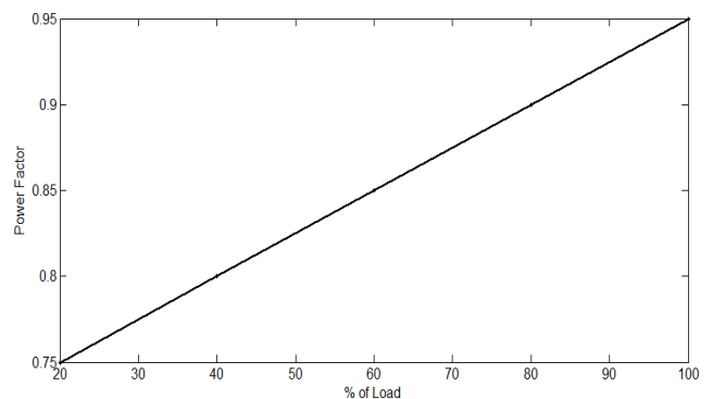
Fig. 13 Power Factor Vs % of Load
