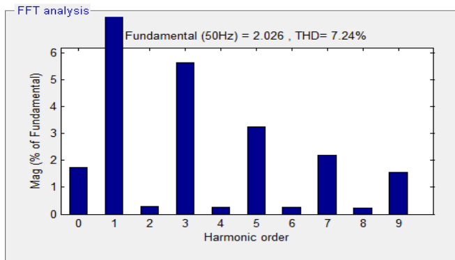
Fig. 10 Supply Current THD
