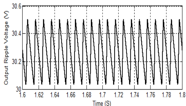
Fig. 7 Output ripple voltage for the proposed IBC
