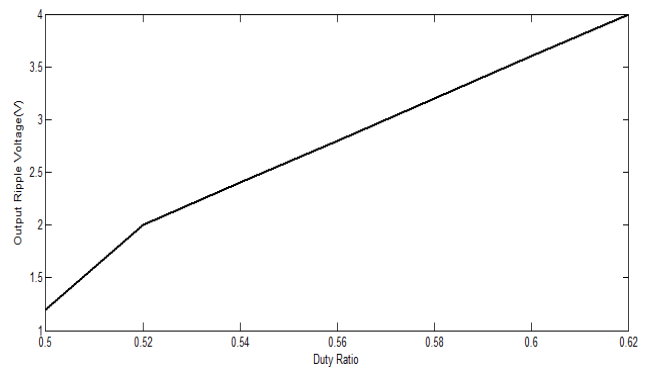
Fig. 11 Output ripple voltage Vs Duty ratio
