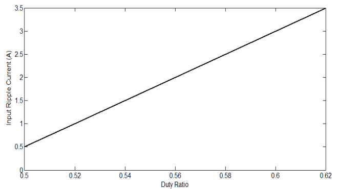
Fig. 12 Input ripple current Vs Duty ratio
