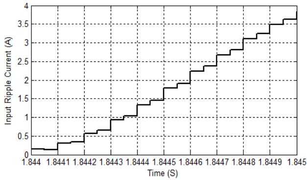
Fig. 8 Input ripple current
