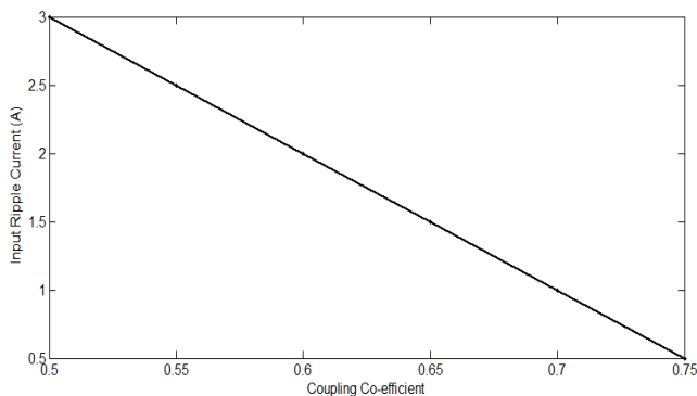
Fig. 14 Input Ripple Current Vs Coupling Co-efficient
