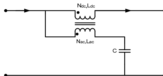
Fig. 1 Coupled inductor with smoothing capacitor
