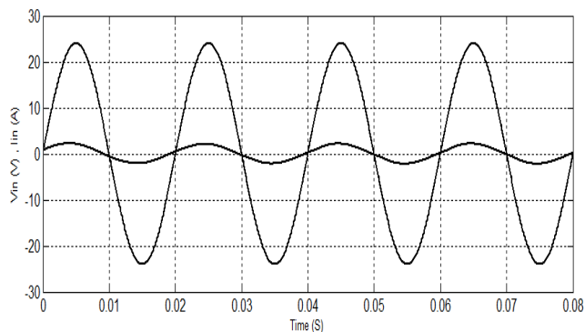
Fig. 4 Supply side Voltage & Current of Coupled IBC
