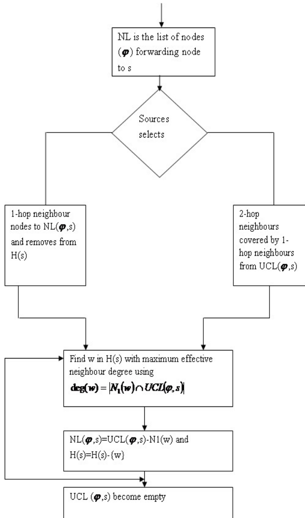
Fig. 2 Flowchart for Finding Forward Node
