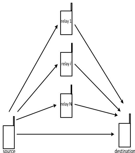
Fig. 1 (b) 3 – node cooperative multi-relay communication scheme
