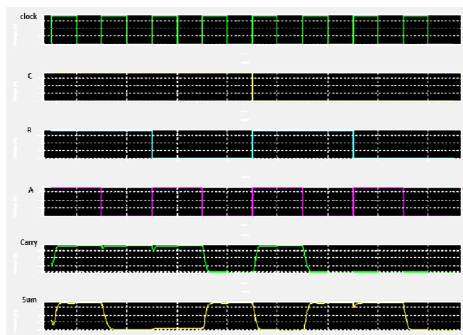
Fig. 3 Simulated output waveform of the TSPC full adder
