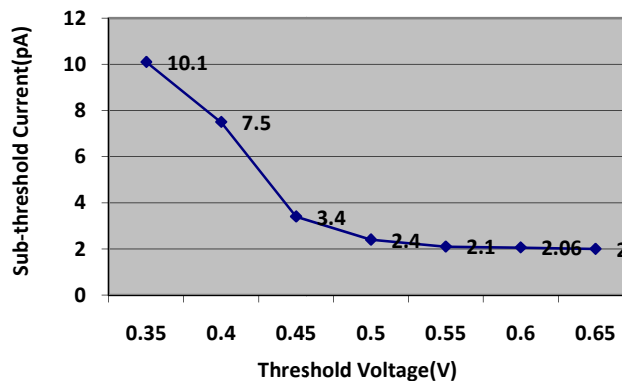
Fig. 5 Variation of Sub-Threshold Current with Threshold Voltage
