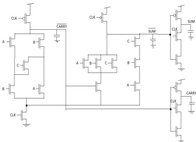
Fig. 2 TSPC full adder circuit
