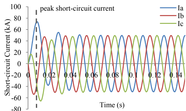
Fig. 4 Three-phase short-circuit current
