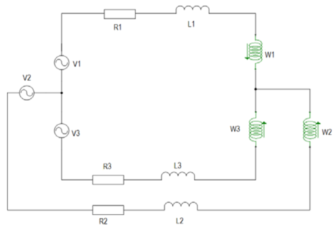
Fig. 3 Equivalent circuit
