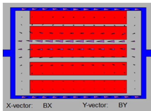
Fig. 8 Vector map of magnetic flux density from Opera-2D
