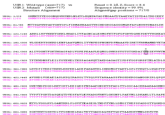
Fig. 2 (c) The structural alignment for the two-modeled domain structure using CE method. In this the * indicates a position that is not conserved (different [S-R]) between WT and mutant KatG
