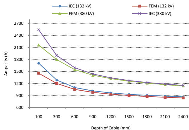
Fig. 2 Ampacity versus depth of cable
