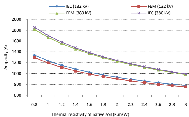
Fig. 3 Ampacity versus thermal resistivity native soil
