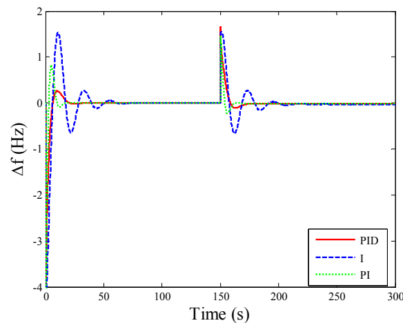
Fig. 16 Simulation results for deviation in frequency in the system with I, PI, PID controller, when load suddenly decreases at 150s
