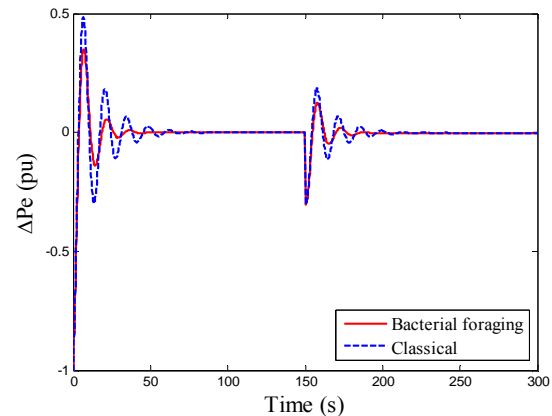
Fig. 4 Simulation results for error in supply demand in the system with I controller, when load suddenly increase
