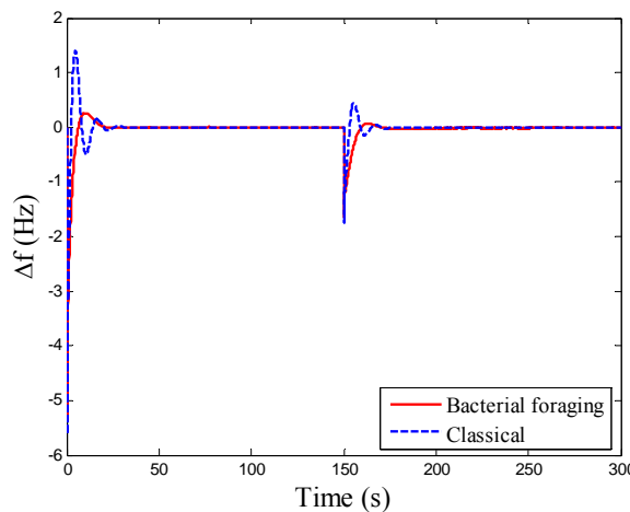
Fig. 11 Simulation results for deviation in frequency in the system with PID controller, when load suddenly increases
