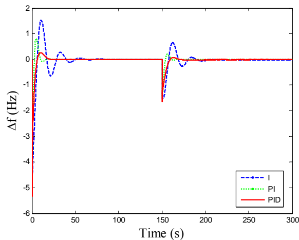
Fig. 15 Simulation results for deviation in frequency in the system with I, PI, PID controller, when load suddenly increases at 150s
