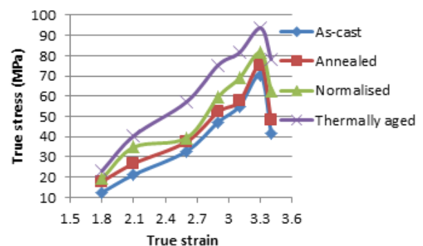
Fig. 2 True stress-strain graph of test specimens
