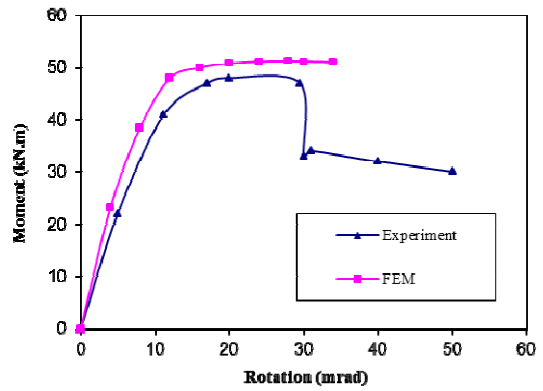
Fig. 6 Moment rotation for EP2
