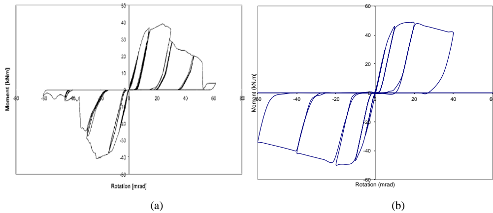
Fig. 8 Moment rotation for EP4: (a) Experimental [3], (b) FEM
