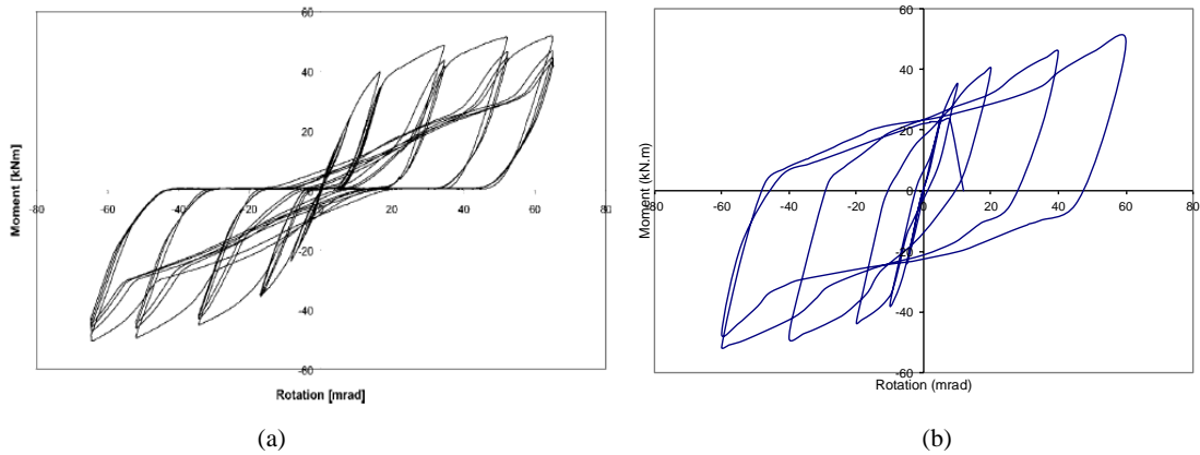
Fig. 7 Moment rotation for EP3: (a) Experimental [3], (b) FEM
