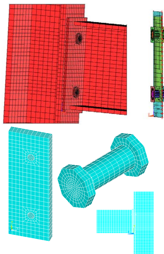
Fig. 2 Model of Flush end plate connection and meshing configuration
