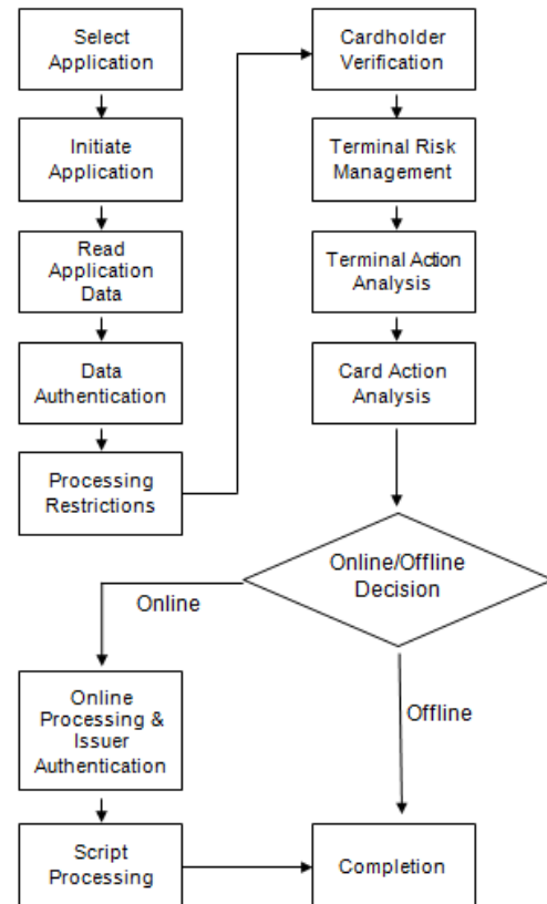
Fig. 1 EMV Work Flow
