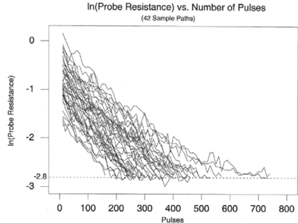
Fig. 2 Sample Degradation Paths on Logarithmic Scale
