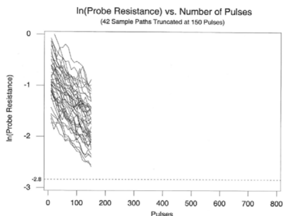
Fig. 8 Sample Degradation Paths Truncated at 150 Pulses
