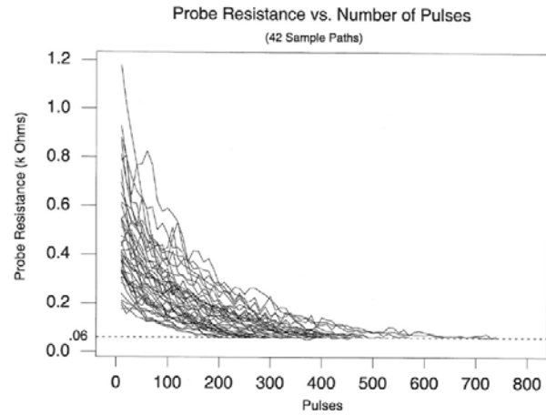
Fig. 1 Sample Degradation Paths
