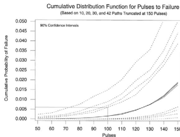
Fig. 9 CDFs Based on Degradation Paths Truncated at 150 Pulses
