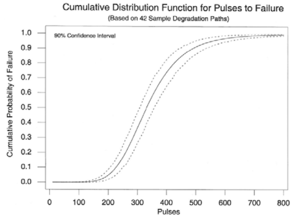
Fig. 4 CDF for Pulses to Failure
