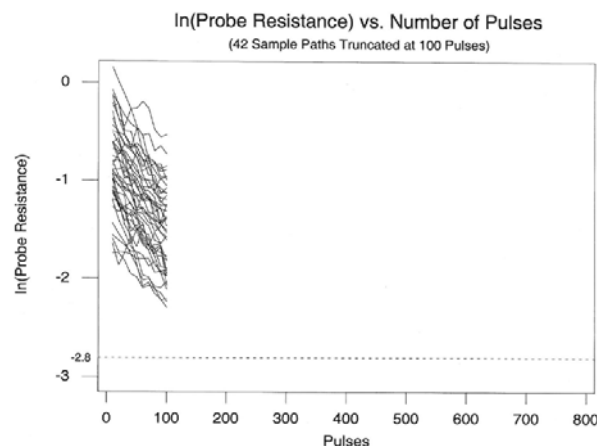
Fig. 6 Sample Degradation Paths Truncated at 100 Pulses
