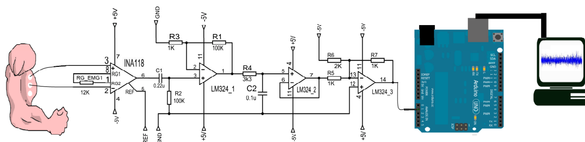
Fig. 1 Electrode configuration (left) followed by the amplification (500x) and band-pass filter (10-500Hz) circuit, the output of this circuit is digitalized by the Arduino microcontroller that export the result to a computer
