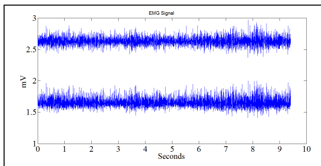
Fig. 6 EMG signal
