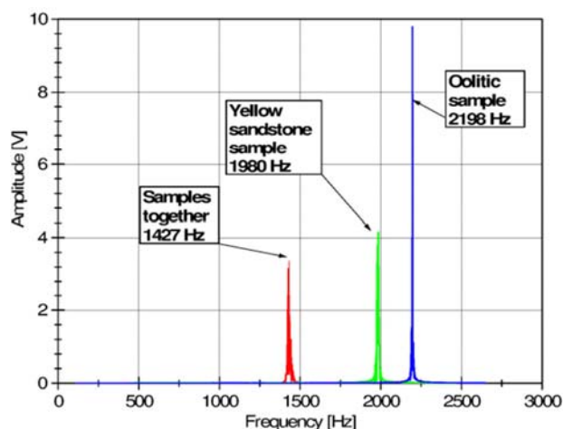
Fig. 5 FFT Frequency spectrum for three kinds of material using SAS system
