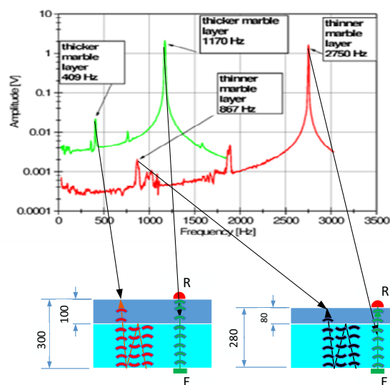
Fig. 7 FFT frequency spectrum for coupled concrete-marble material in two configuration of marble thickness
