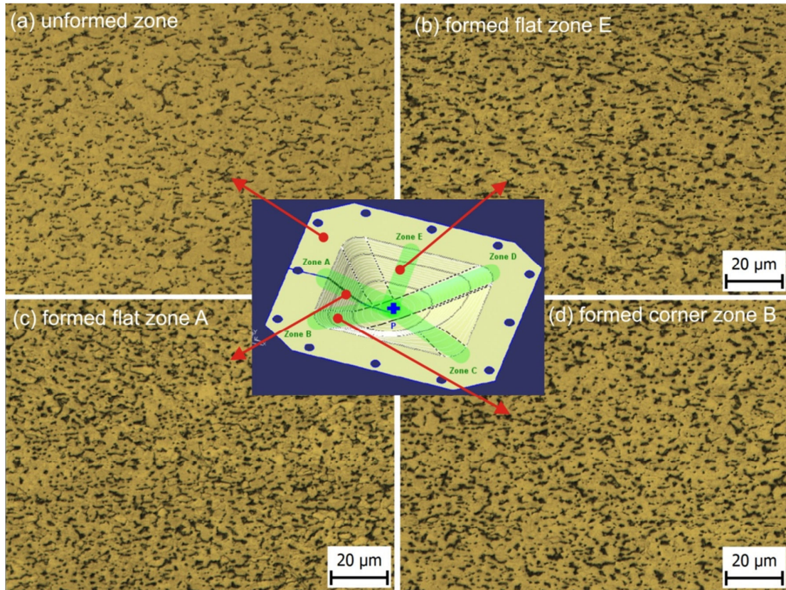
Fig. 5 Microstructure of the Ti-6Al-4V alloy in different zones AISF formed part. Etched by the Kroll's reagent (magn. 1000×)
