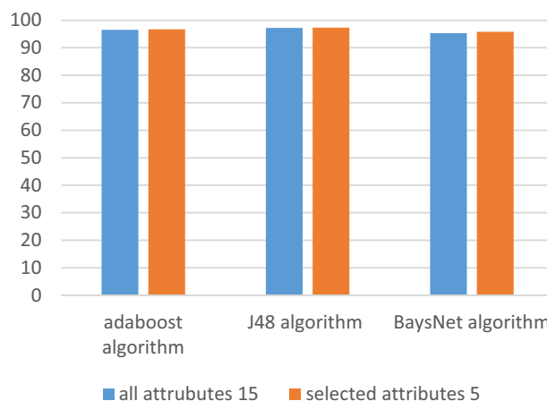
Fig. 3 Comparison Accuracy Results between using all attributes and selected 5 attributes
