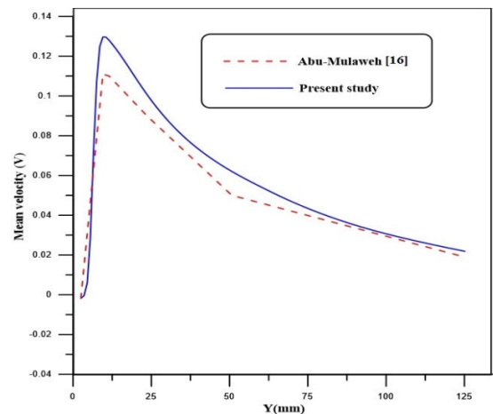
Fig. 2 Comparison of velocity profile with [16]
