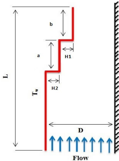
Fig. 1 Geometry model
