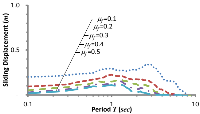
Fig. 5 Sliding displacement
