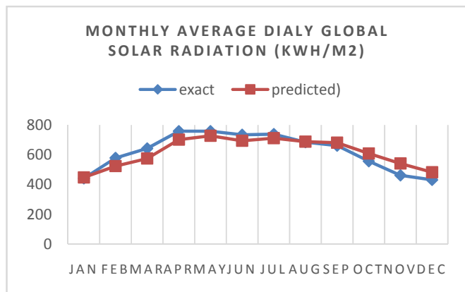
Fig. 4 Monthly average daily global solar radiation estimation of model MLP 4-12-1
