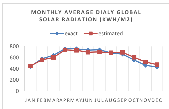
Fig. 5 Monthly average daily global solar radiation estimation of model RNN 5-4-1
