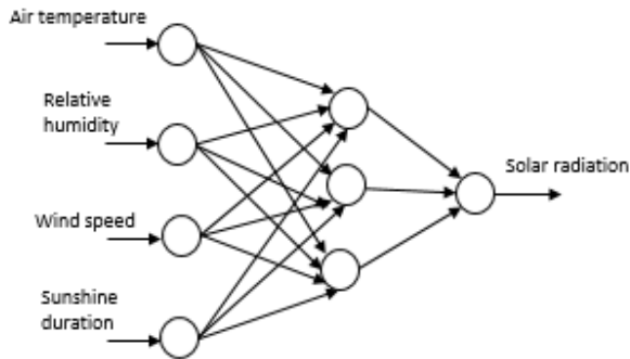
Fig. 2 The fully connected MLP used in the reference estimation system
