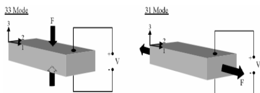
Fig. 6 Coupling modes of piezoelectric material
