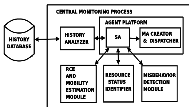
Fig. 3 Architecture of main process of node monitoring protocol
