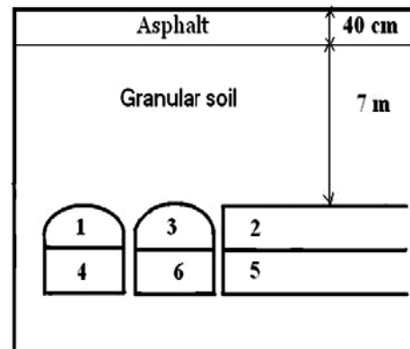
Fig. 7 Construction procedure D (Method D)
