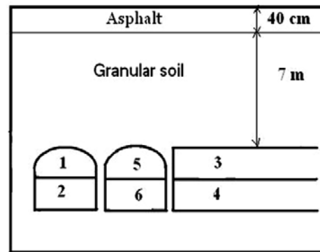
Fig. 6 Construction procedure C (Method C)
