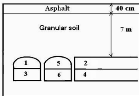
Fig. 5 Construction procedure B (Method B)
