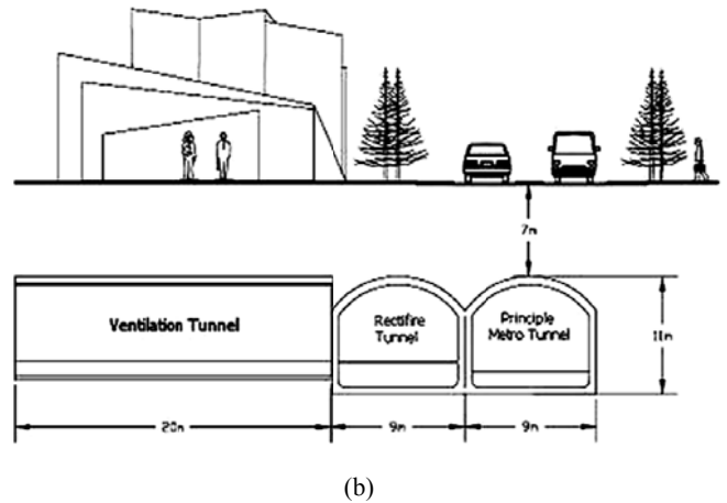
Fig. 1 Arrangement of tunnels: a) plan, b) section a-a
