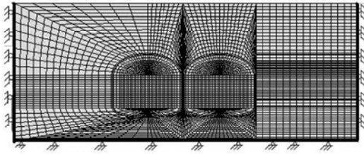
Fig. 4 Mesh used in the analysis of tunnels
