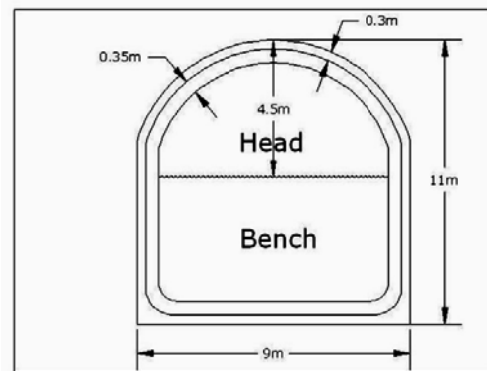
Fig. 2 Tunnel geometry
