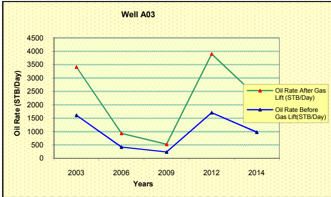
Fig. 3 Output design results of well A03
