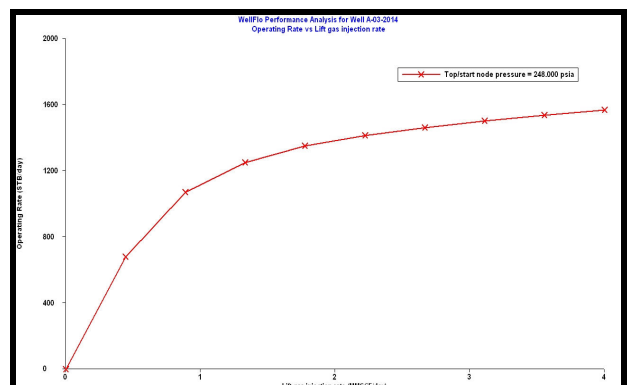
Fig. 7 Lift gas injection rate and Top/Start node pressure on Inflow/Outflow Curve of well A03 for year 2014
