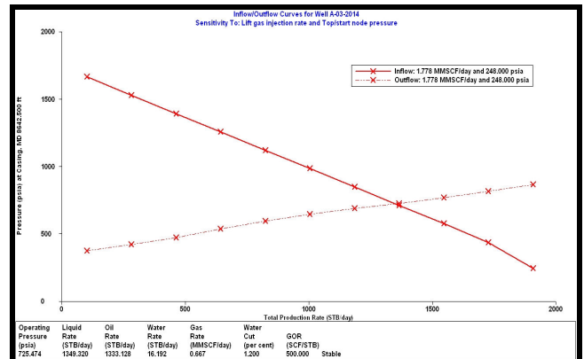
Fig. 6 Optimization lift gas injection rate of well A03 for year 2014
