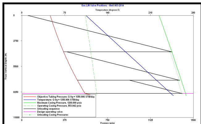
Fig. 8 Gas lift valve position of well A03 for year 2014
